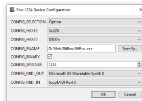
Fig. 1: All option types currently configurable through the user interface. [TO BE UPDATED ONCE I GET OUT OF HIDPI]
